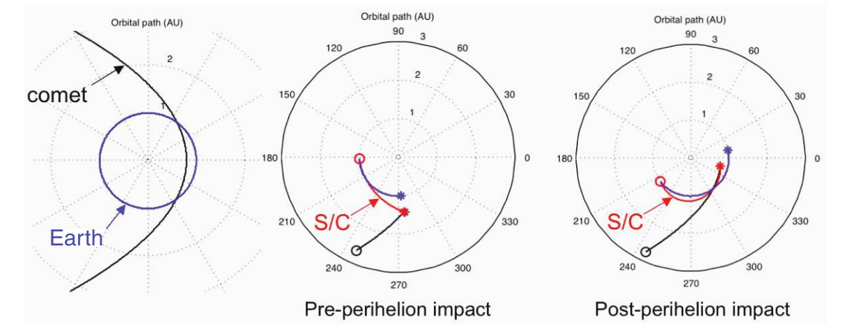
FIGURE 5.4 Intercept trajectories for a hazardous, long-period comet. The left panel shows the comet’s orbit and the two places at which it intercepts Earth’s orbit. The next two panels show the intercept trajectories corresponding to the two rows in Table 5.6. In other respects, the panels are similar to those in Figure 5.3.
